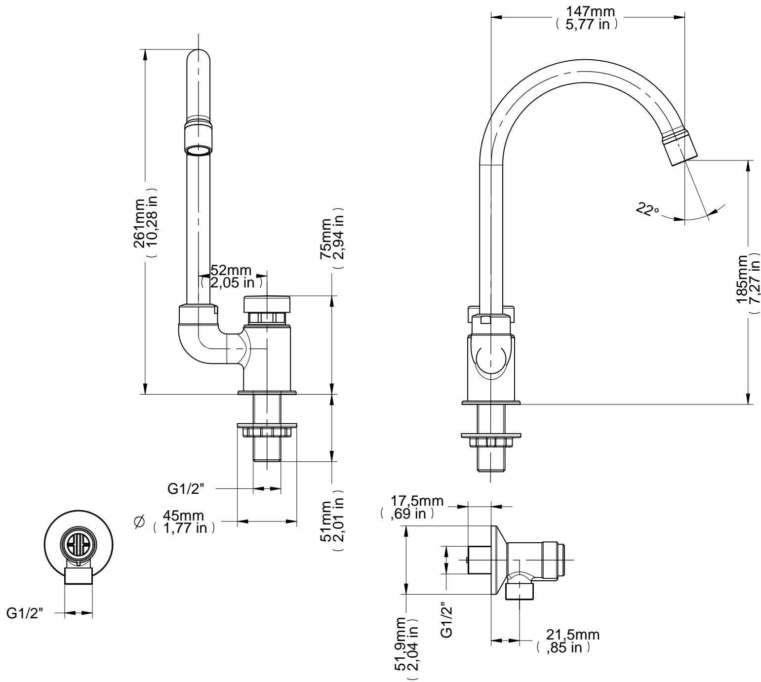
TORNEIRA MESA LAVATORIO PRESSMATIC BICA ALTA - DN 1/2" ALFA BASIN PILLAR TAP - HIGH SPOUT - 1/2" GRIFO MESA PICO ALTO - 1/2"
