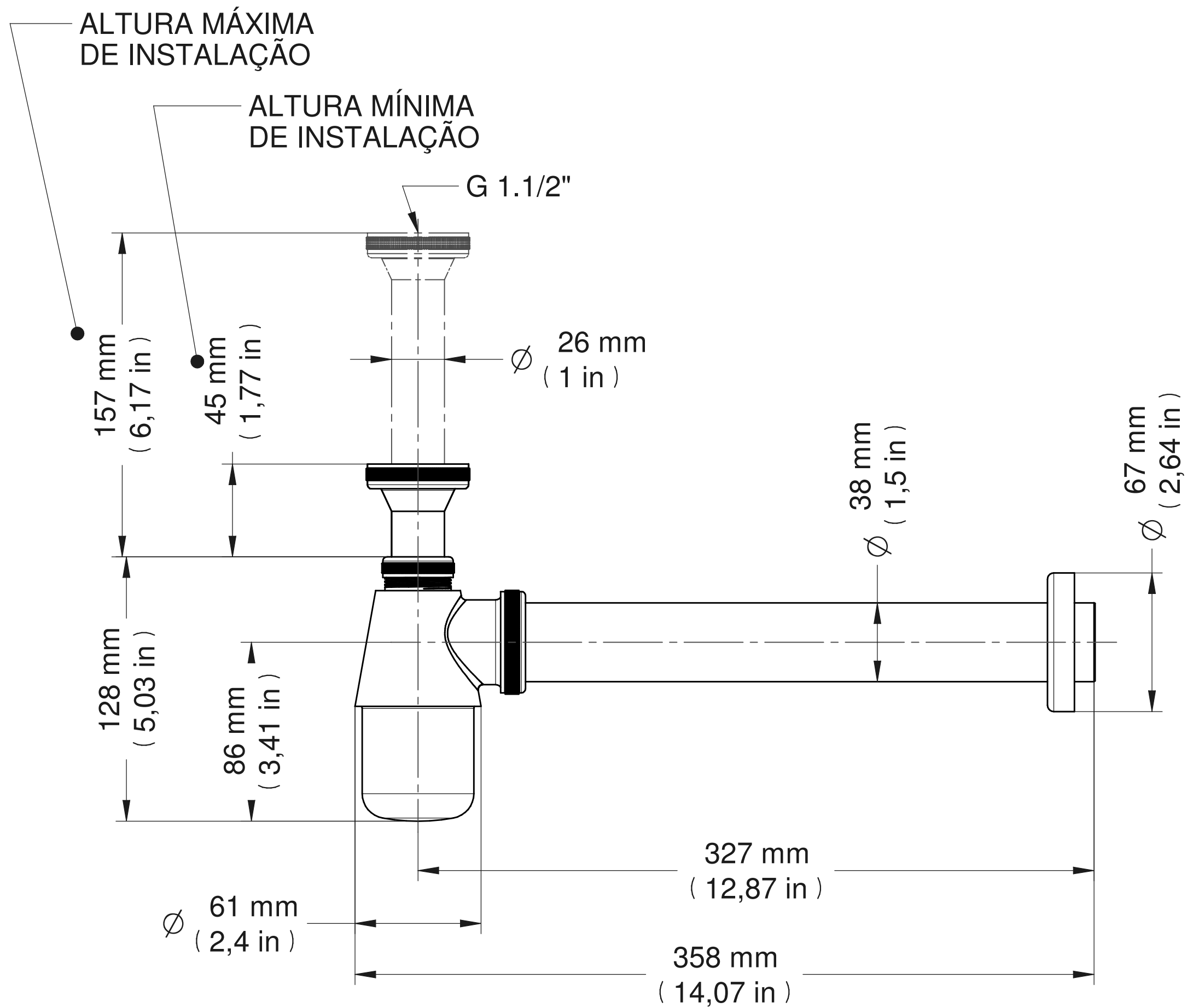
SIFAO PARA COZINHA STANDARD - ENTRADA G1.1/2"- SAIDA TUBO DN40(38,1) - CR STANDARD KITCHEN TRAP - INLET G1.1/2" - OUTLET PIPE DN40(1.1/2") - CR SIFON COCINA STANDARD - ENTRADA G1.1/2"- SALIDA TUBO DN40(1.1/2") - CR
