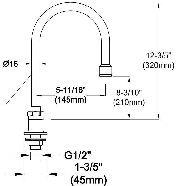
P-0133 gooseneck nozzles
